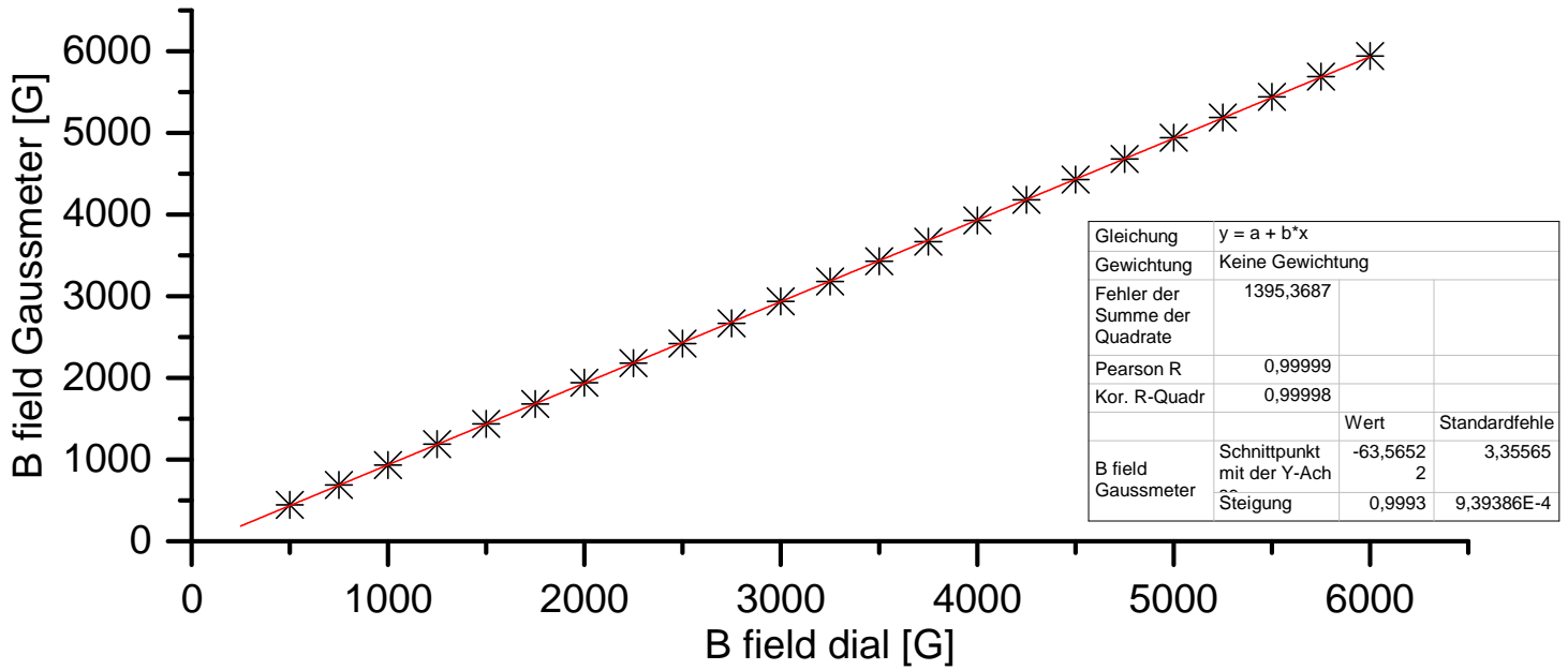
Deviation of set B field on dial and Gaussmeter placed between magnet poles
